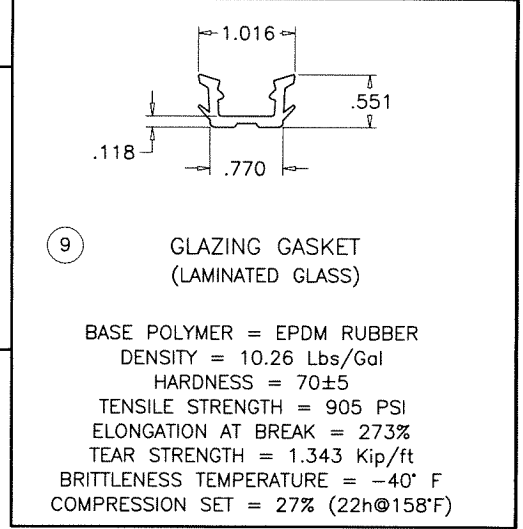
FIXED PANEL CLIP
